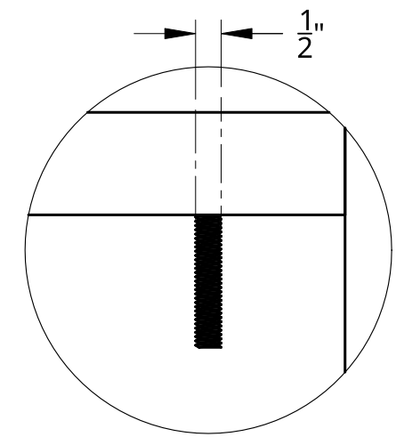
DETAIL A 1/2" Hole SCALE 1:5
